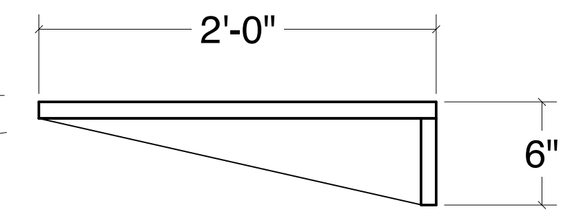
3/8" bent plate with stiffener & wedge anchor @ 12" O/C
