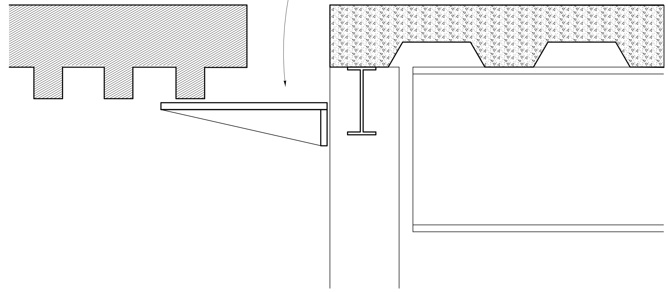
Detail B 1/2" = 1'
