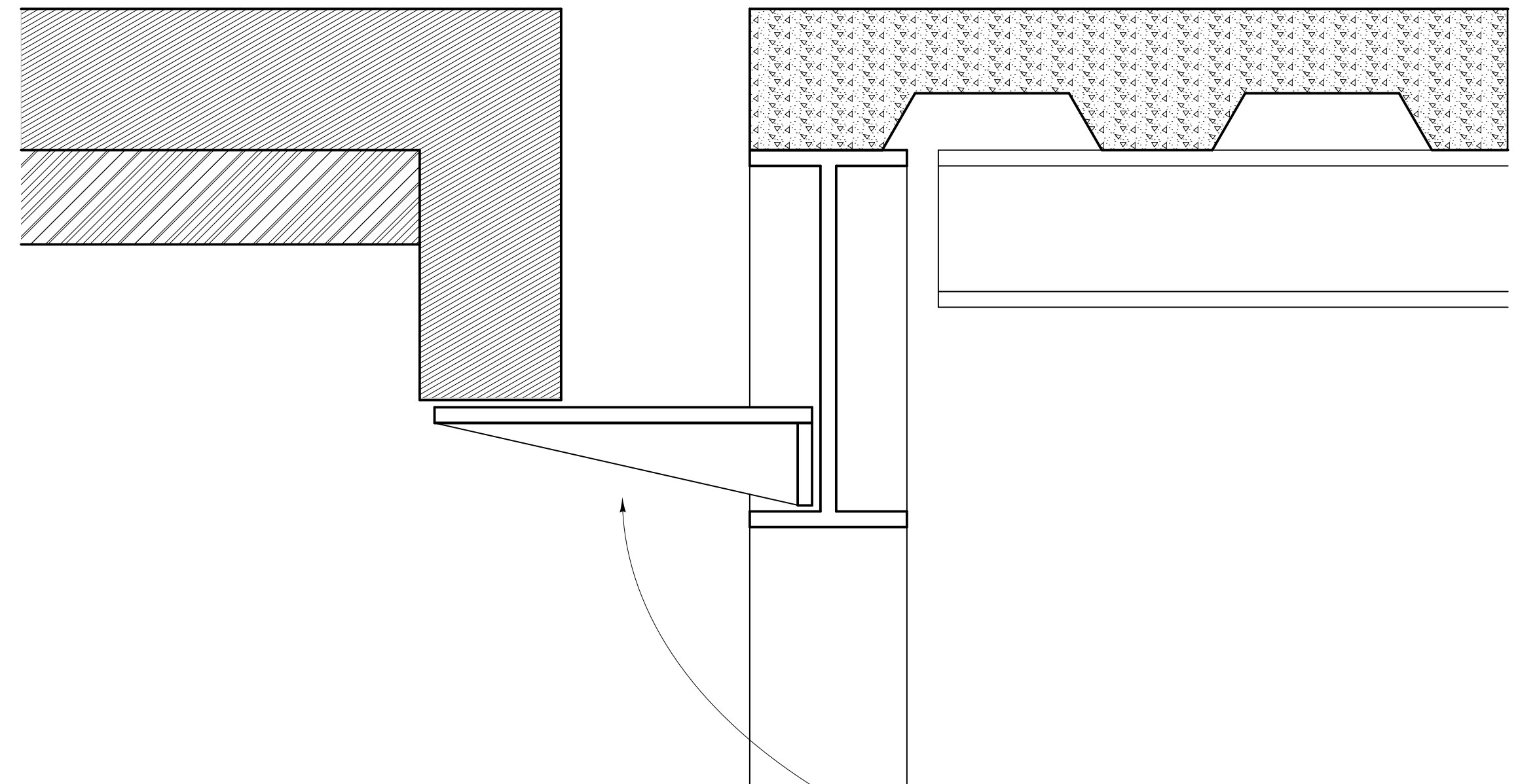
Detail A 1/2" = 1'
