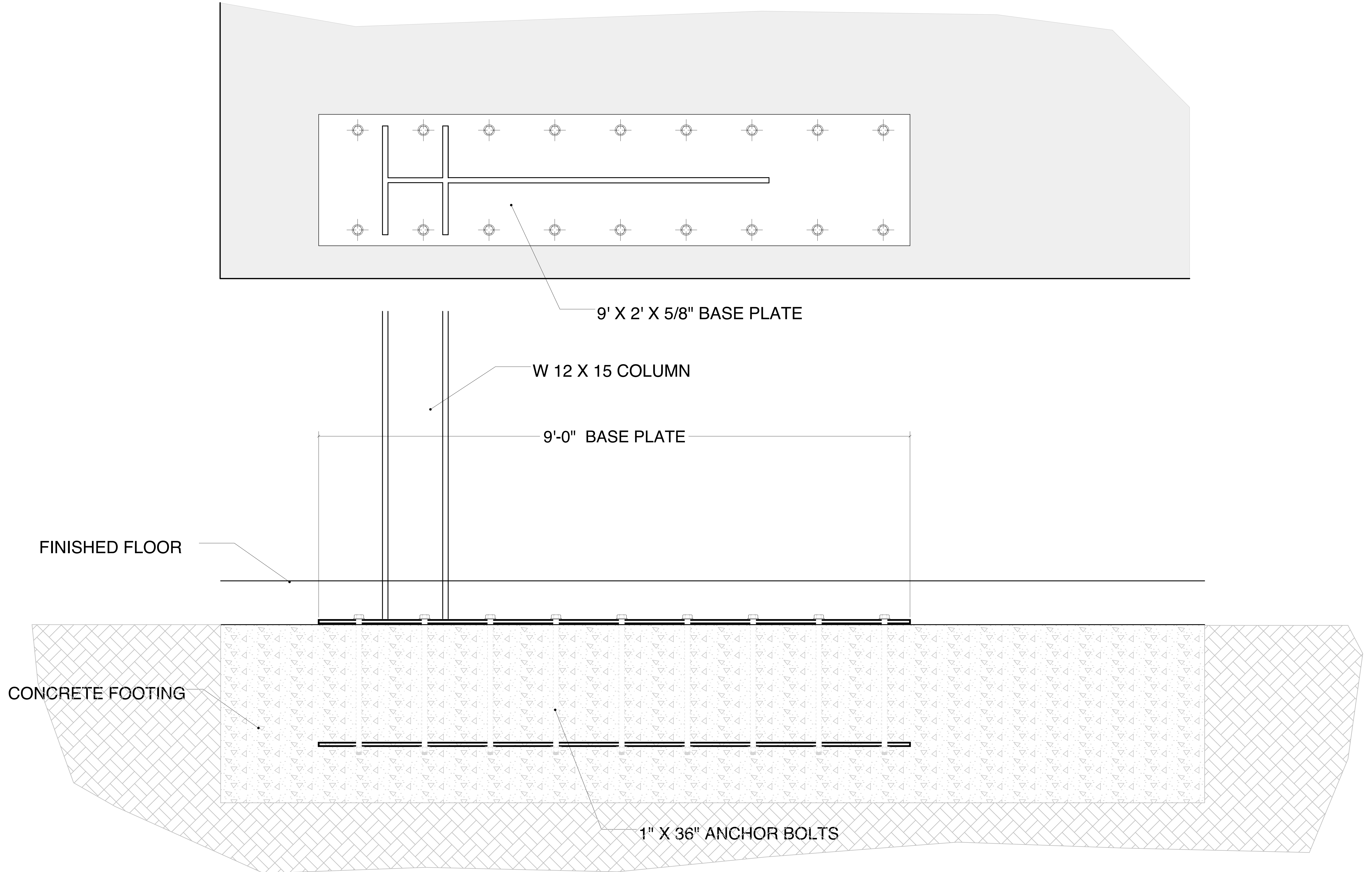
COLUMN / PLATE BASE PLATES 1 1/2" = 1'
