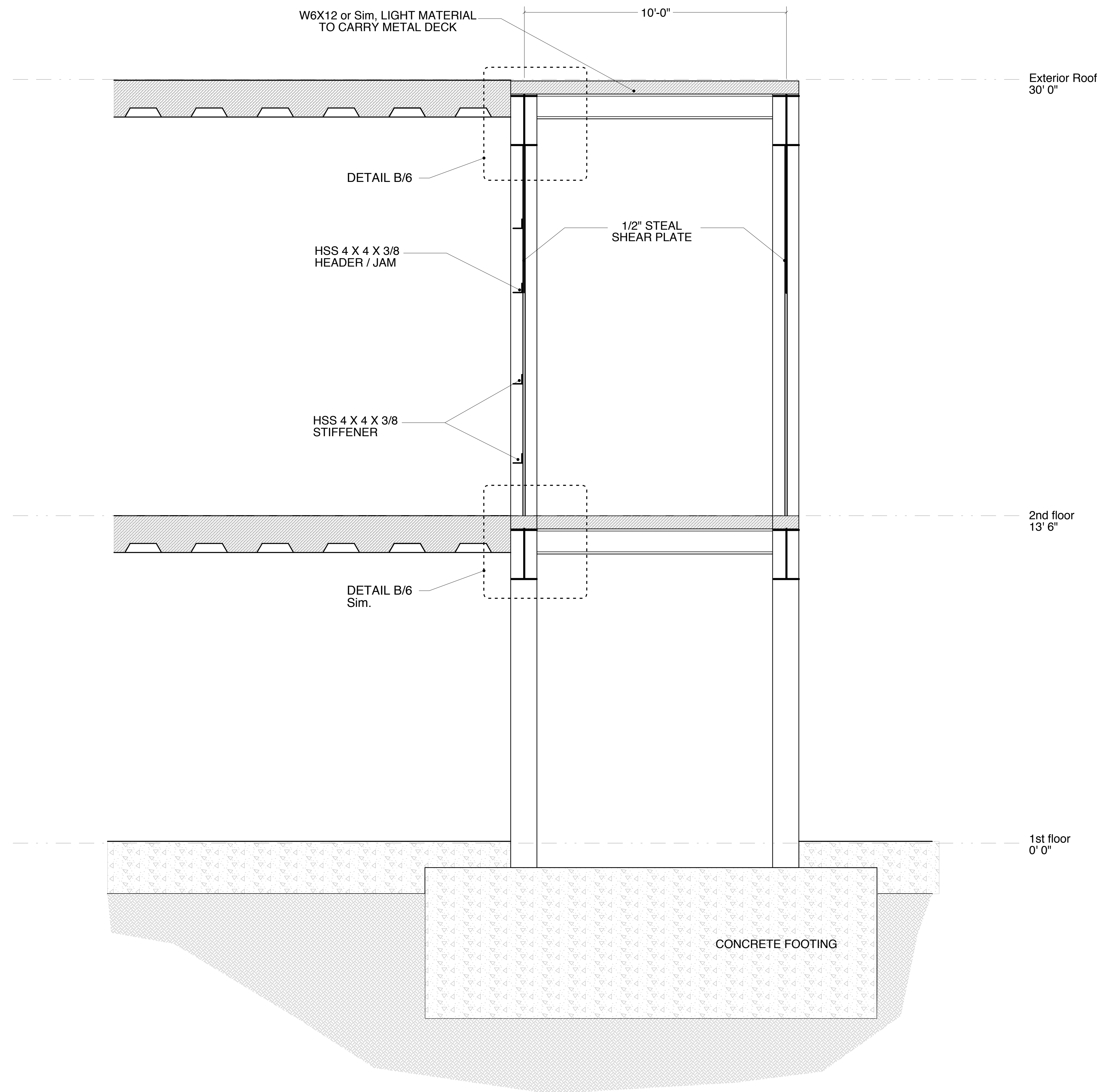
Section B 1/2" = 1'
