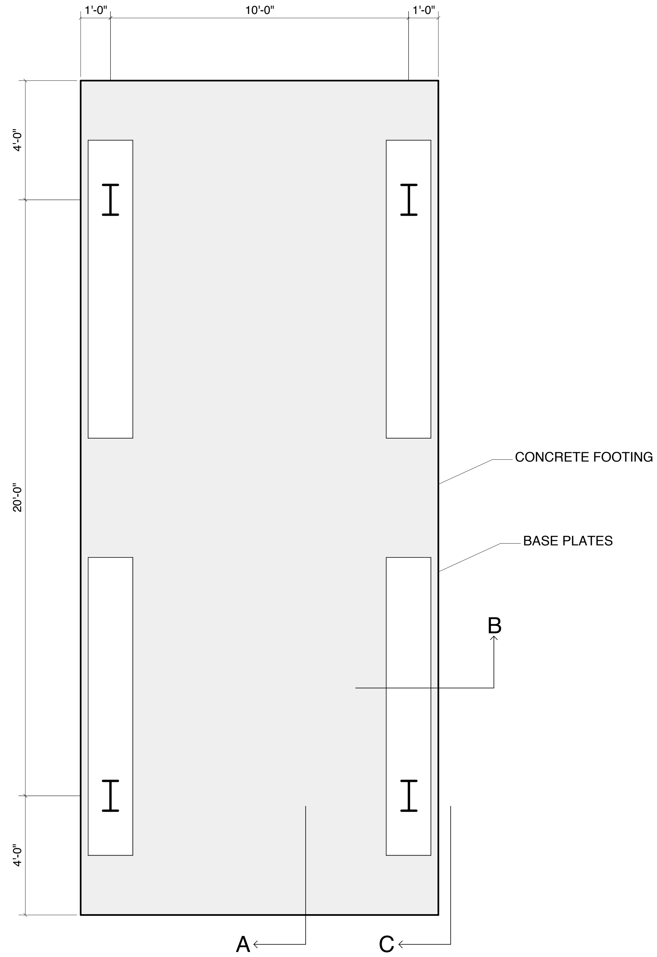
FOUNDATION PLAN 1/2" = 1'
